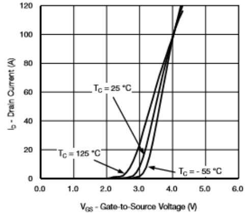
Transfer Characteristics
