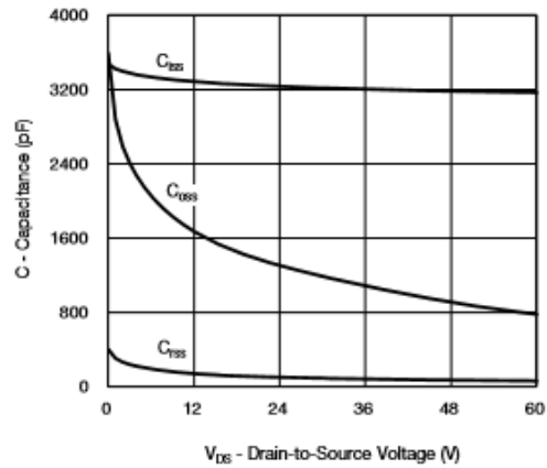
Capacitance
