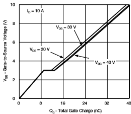
Gate Charge
