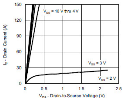
Output Characteristics
