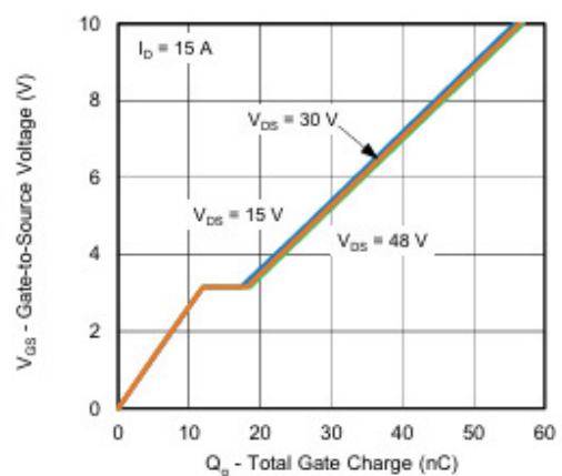
Gate Charge
