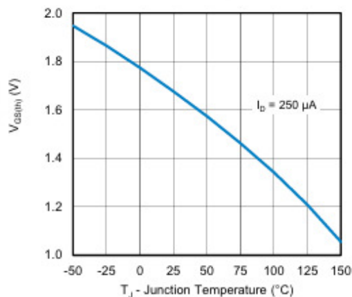
Threshold Voltage
