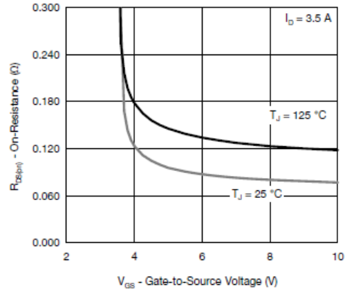
R_{DS(on)} vs. V_{GS} vs. Temperature
