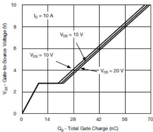
Q_g - Total Gate Charge (nC) Gate Charge
