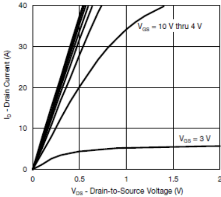
Output Characteristics
