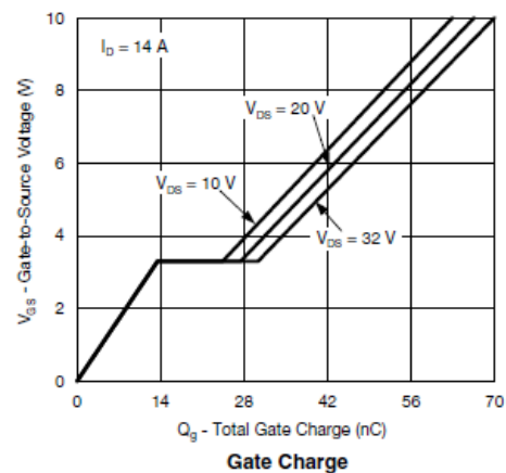
Gate Charge
