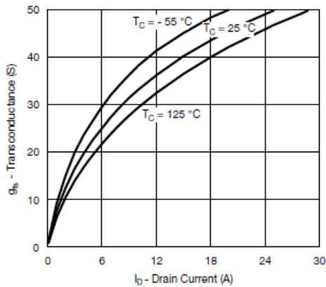
Transconductance
